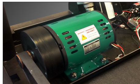
5.0 HP, AC NextGEN III Eco-Drive System™
